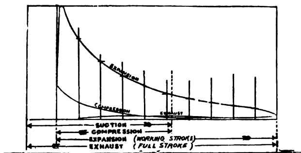
FIG. 305.—Indicator Card for the Atkinson Variable Stroke Four-Part "Two-Cycle" Gas Engine.
